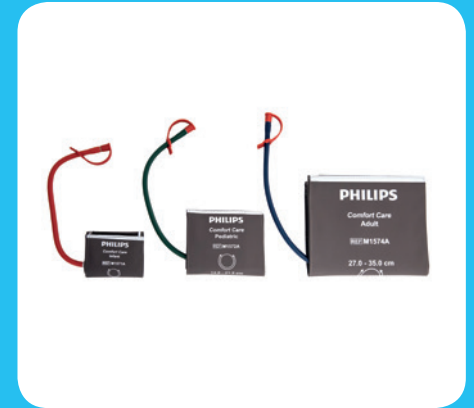
Blood pressure
